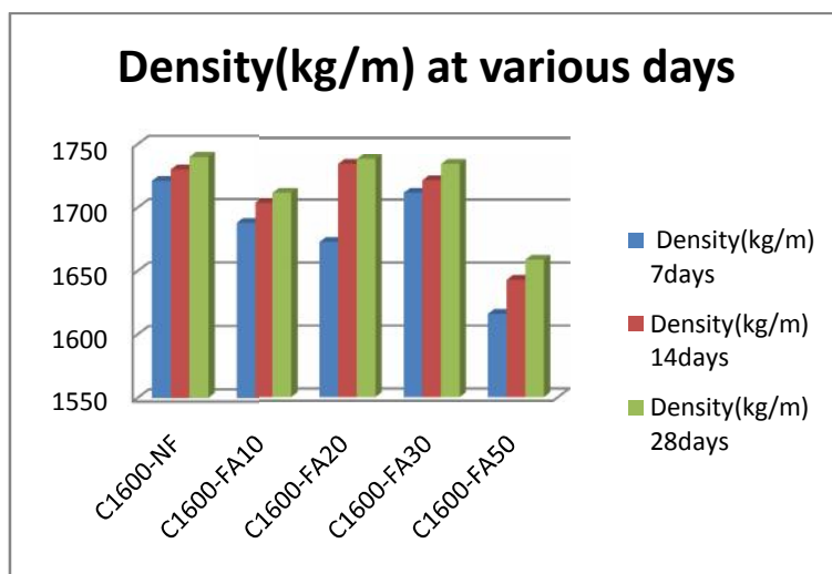
Fig. 1 Shows the density at various test age.
